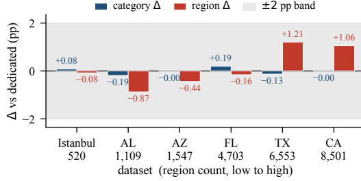
Fig. 3. Signed differences between the joint model and the dedicated single-task models, ordered by region count. Every difference falls inside the \pm 2 -point band, which applies to region only. The region difference (Acc@10) is clearly positive at Texas and California, the two largest region vocabularies, and slightly negative at the other four; the category difference (macro-F1) stays within a fifth of a point everywhere.
